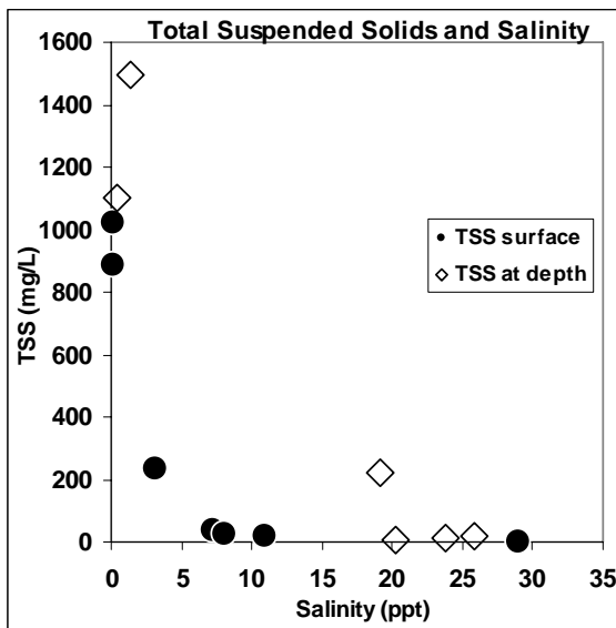
Figure 5. TSS concentrations for surface and depth (below plume) samples, and salinity (salinity increasing from sites 1 to site 7)
