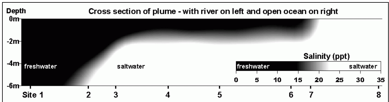
Figure 4. Map of flood plume (not to scale, Y axis [depth] is exaggerated) site 3 is river mouth
