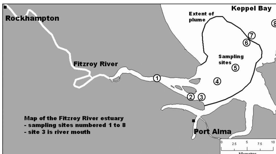
Figure 3. River, estuary and plume sampling sites for the February 2003 Fitzroy River flood
