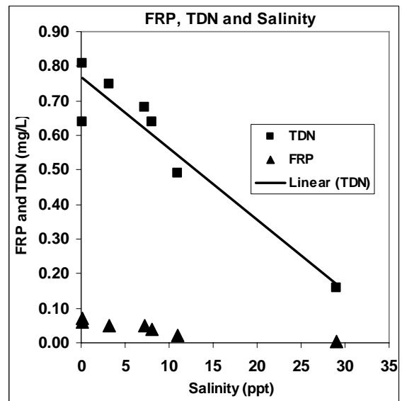
Figure 6. Filterable Reactive Phosphorus (FRP) and Total Dissolved Nitrogen (TDN) concentrations (surface only), and salinity
