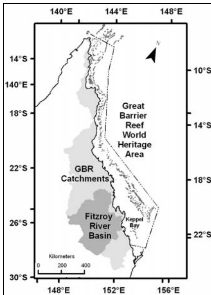
Figure 1. Great Barrier Reef Catchments and the Fitzroy River Basin
