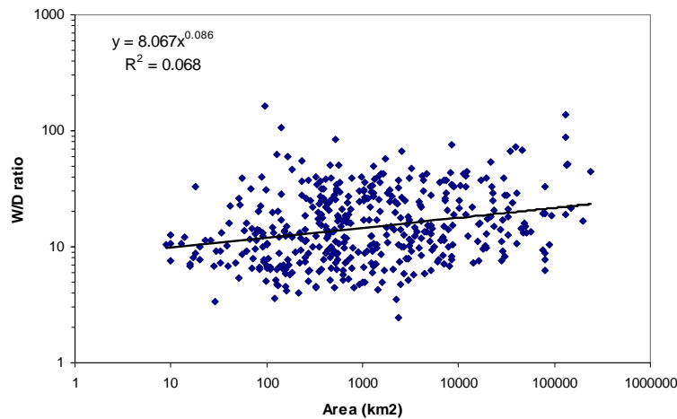
Figure 1 Variation in W/D ratio with increasing catchment area for surveys in the State of Rivers database.
